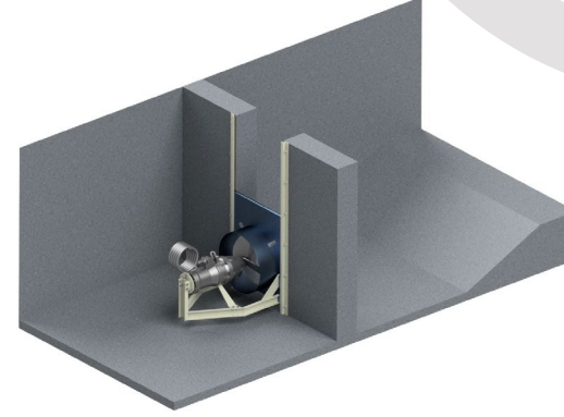
Sirkülasyon Kaidesi - Z Tip Circulations Frame - Mounting in Z-Splint
