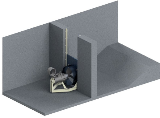
Sirkülasyon Kaidesi - U Tip Circulations Frame - Mounting in U-Splint
